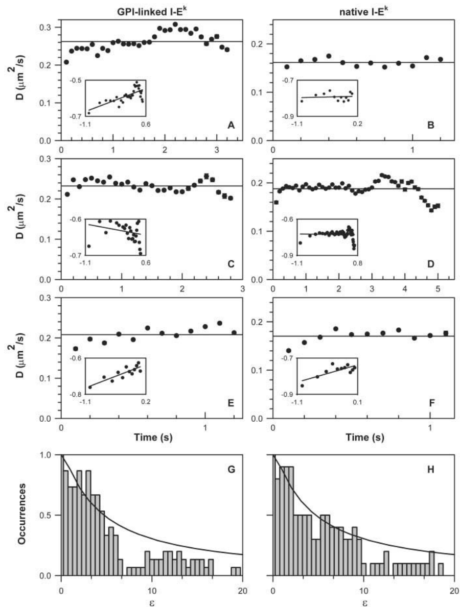
FIGURE 5 Influence of actin and tubulin depolymerization on the diffusion of GPI-linked and native I-E k proteins. (A) Actin disruption for GPI-linked I-E k . Data are shown for 40 μM cytochalasin D, 30 min, 37°C. The same effect was observed for 10 μM cytochalasin D. Under white light cells are spherical, not spindly, indicating that stress fibers are depolymerized (see Materials and Methods). Shown are diffusion coefficients as a function of time. All other parameters as in Fig. 2 C; 104 trajectories were analyzed (from 10 cells) (average length 3.2 s). The mean value of D = 0.26 \pm 0.024 \mu\text{m}^2/\text{s} . Error bars for each D represent standard error from the fit to Eq. 1 for each respective time lag. Inset: \alpha = 1.07 \pm 0.014 , D_0 = 0.26 \pm 1.3 \times 10^{-3} \mu\text{m}^2/\text{s} . (B) Actin disruption for native I-E k . Experimental conditions and fit parameters as in A; 52 trajectories (from 9 cells) were analyzed, average length 3.2 s. Mean value of D = 0.16 \pm 7.8 \times 10^{-3} \mu\text{m}^2/\text{s} . Inset: \alpha = 1.0 \pm 0.020 , D_0 = 0.16 \pm 1.4 \times 10^{-3} \mu\text{m}^2/\text{s} . (C) Tubulin disruption for GPI-E k . Under white light cells are not as spindly as controls and look flattened, suggesting that the tubulin network has depolymerized (see Materials and Methods). Shown are diffusion coefficients as a function of time for 77 trajectories (from 10 cells), average length 2.9 s. All other parameters as in Fig. 2 C. Mean value of D = 0.23 \pm 0.015 \mu\text{m}^2/\text{s} . Inset: \alpha = 0.98 \pm 0.014 , D_0 = 0.23 \pm 1.2 \times 10^{-3} \mu\text{m}^2/\text{s} . (D) Tubulin disruption for native I-E k , same as C; 123 trajectories were analyzed (from 14 cells), average length 5.1 s. The mean value of D = 0.19 \pm 0.016 \mu\text{m}^2/\text{s} . Inset: \alpha = 0.99 \pm 0.014 , D_0 = 0.19 \pm 1.3 \times 10^{-3} \mu\text{m}^2/\text{s} . (E) GPI-linked I-E k , 4 μl DMSO, 30 min, 37°C. All other parameters as in A; 51 trajectories were analyzed (from 6 cells), average length 2.7 s. The mean value of D = 0.21 \pm 0.018 \mu\text{m}^2/\text{s} . Inset: \alpha = 1.10 \pm 0.019 , D_0 = 0.22 \pm 0.018 \mu\text{m}^2/\text{s} . (F) Native I-E k , Same as E; 37 trajectories were analyzed (from 7 cells), average length 3.3 s. The mean value of D = 0.17 \pm 0.013 \mu\text{m}^2/\text{s} . Inset: \alpha = 1.08 \pm 0.023 , D_0 = 0.18 \pm 1.8 \times 10^{-3} \mu\text{m}^2/\text{s} . (G) Actin disruption for GPI-linked I-E k . Shown is the correlation in diffusion of the "pairs." All parameters as in Fig. 4 D; 12 pairs (from 5 cells) longer than 2 s were analyzed. (H) Actin disruption for native I-E k . Experimental conditions and fit parameters as in G; 6 pairs (from 2 cells) longer than 3.7 s were analyzed.
